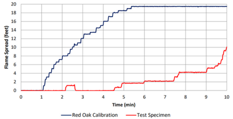
Graph 1: Flame Spread Index (FSI)
